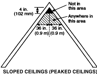
SLOPED CEILINGS (PEAKED CEILINGS)
