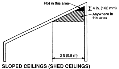
SLOPED CEILINGS (SHED CEILINGS)
